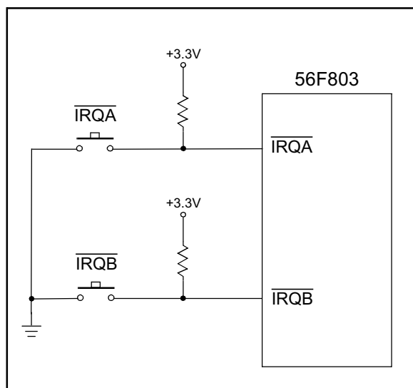
Figure 2-6. Schematic Diagram of the User Interrupt Interface
