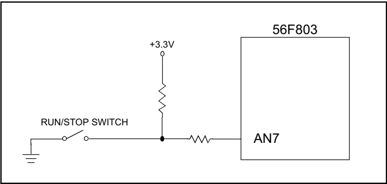
Figure 2-9. Run/Stop Switch
