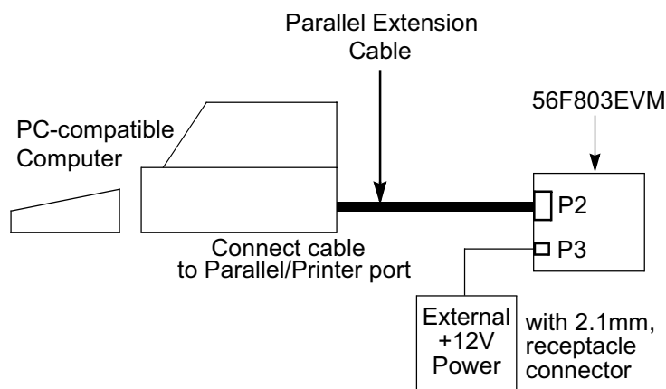
Figure 1-3. Connecting the 56F803EVM Cables
