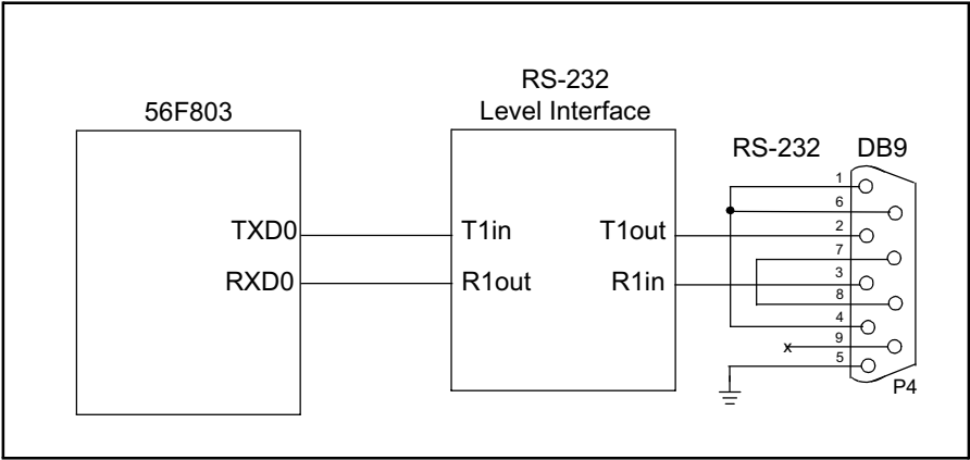
Figure 2-2. Schematic Diagram of the RS-232 Interface
