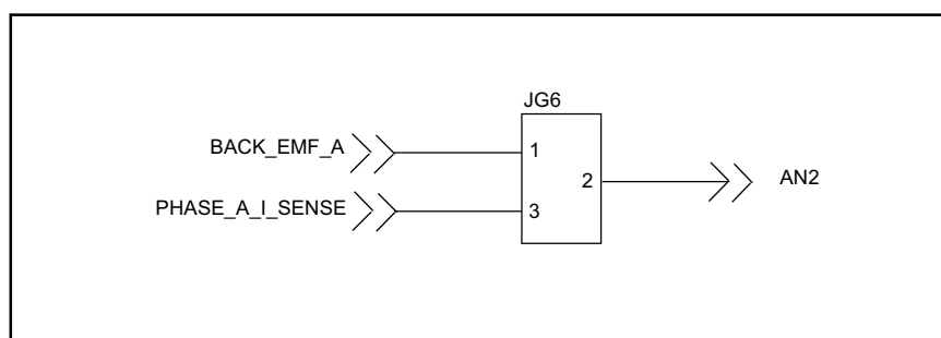
Figure 2-12. Primary Back-EMF or Motor Phase Current Sense Signals
